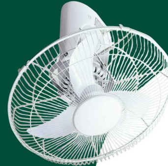
Model No.: RO-1602 16" Rechargeable orbit fan DC motor, 12V 12W 12V5Ah lead acid battery or lithium-ion battery Duration: 5-12hrs With wall control & remote control Option for Solar panel Single packing size: 43*13*48.5CM 2pcs/color box, 3064pcs/40'HQ
